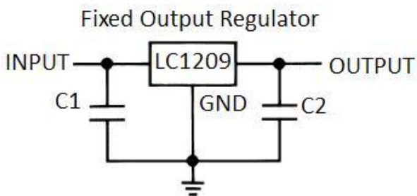
Application circuit of LC1209
